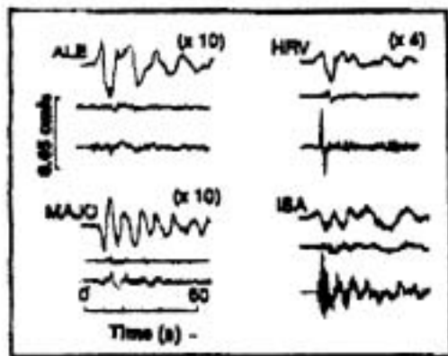
Fig. 4. Broad-band velocity records from four stations (ALE, epicentral distance \Delta = 5188 km, azimuth = 9^\circ ; HRV: \Delta = 4368 km, azimuth = 69^\circ ; MAJO: \Delta = 8029 km, azimuth = 308^\circ ; ISA: \Delta = 748 km, azimuth = 132^\circ ) for the main shock (top trace) and the first (middle) and second (lower) aftershocks. The amplitudes of the seismograms at ALE, HRV, and MAJO are increased relative to ISA for display. The large amplitudes of the second aftershock relative to the other two events in the along-strike azimuth (ISA) is attributable to rupture directivity.
